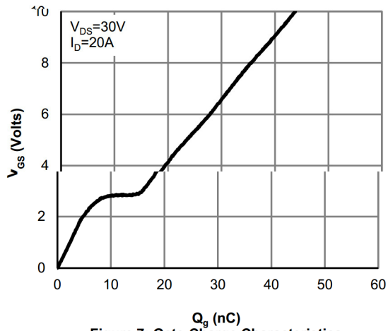
Figure 7: Gate Charge Characteristic Figure 8: Capacitance Characteristic
