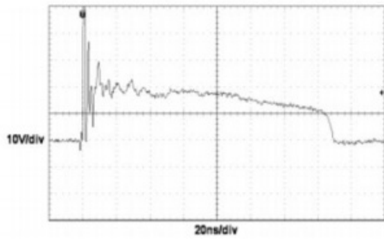
ESD clamping (+8kV contact discharge per IEC 61000-4-2) ESD clamping (-8kV contact discharge per IEC 61000-4-2)
