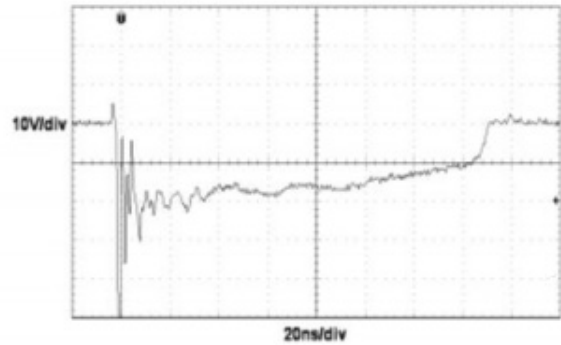
ESD clamping (+8kV contact discharge per IEC 61000-4-2) ESD clamping (-8kV contact discharge per IEC 61000-4-2)
