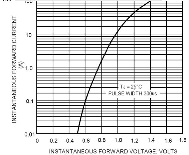
FIG.4-TYPICAL FORWARD CHARACTERISTICS
