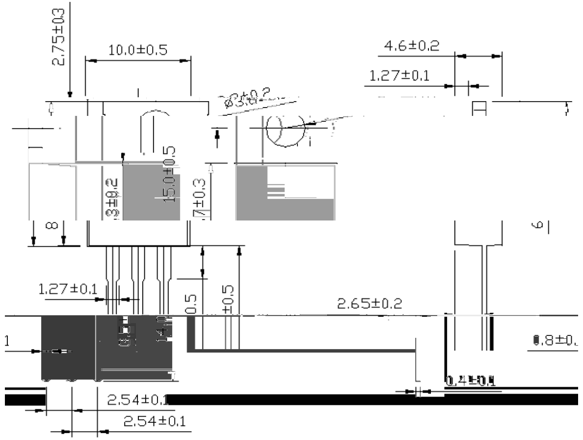
Dimensions in millimeters (1mm =0.0394")
